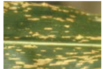
Southern Corn Leaf Blight
